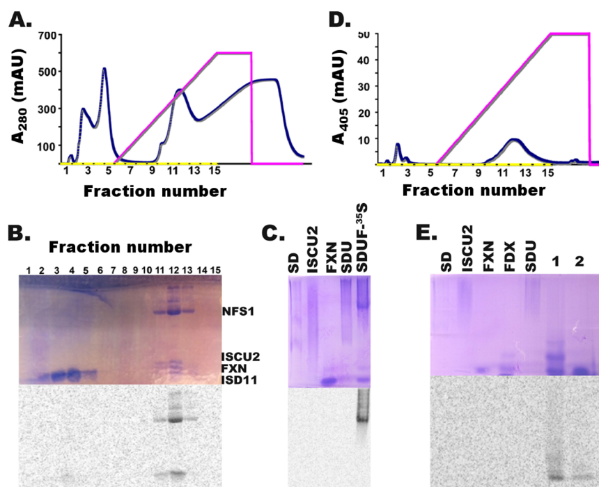
Figure 4. ^{35}\text{S} radiolabel tracking from a cysteine substrate to a Fe-S cluster on FDX. The SDUF complex was reacted (see Experimental Procedures) with L- ^{35}\text{S} cysteine and (A) fractionated with a HisTrap column. (B) Fractions were analyzed for protein (top) and radioactivity (bottom) via nonreducing 14% SDS-PAGE, and (C) fractions 11–13 corresponding to ^{35}\text{S} SDUF were combined and analyzed for protein (top) and radioactivity (bottom) via nonreducing 6.5% Native PAGE. ^{35}\text{S} SDUF was then reacted with iron (see Experimental Procedures) and (D) fractionated on a second HisTrap column. (E) Fractions 2 and 3 from panel D were combined and analyzed via native PAGE in the absence (labeled 1) and presence (labeled 2) of DTT. Standards SD, ISCU2, FXN, FDX, and SDU were included for the native gels; proteins were stained using Coomassie blue, and radioactivity was detected using a Phosphorimager. The absorbance (blue) at 280 (A) or 405 nm (D) was overlaid with a 5 to 500 mM imidazole gradient (pink).
